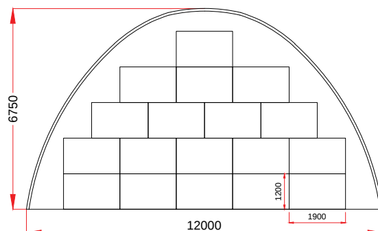
18 x (1.90 m x 1.20 m)
