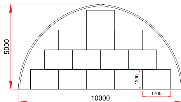
13 x (1.70 m x 1.20 m)
