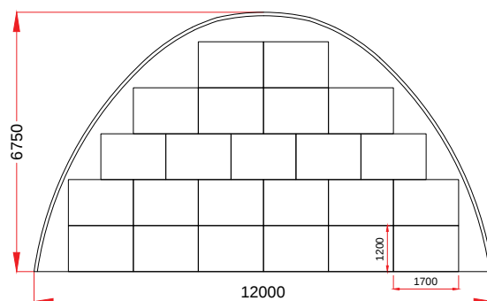
23 x (1.70 m x 1.20 m)
