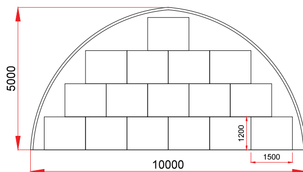
16 x (1.50 m x 1.20 m)
