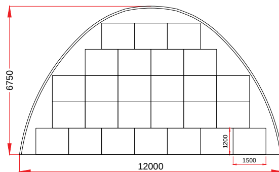
26 x (1.50 m x 1.20 m)
