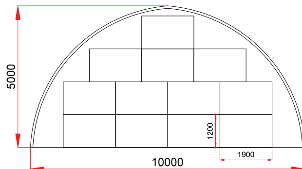
12 x (1.90 m x 1.20 m)
