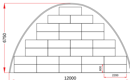
27 x (2.20 m x 0.80 m)
